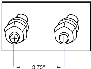
Bolt Pattern for Spring Loaded Light Bars
