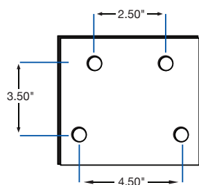
Bolt Pattern Rigid Mount Light Bars
