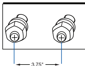
Bolt Pattern for Spring Loaded Light Bars
